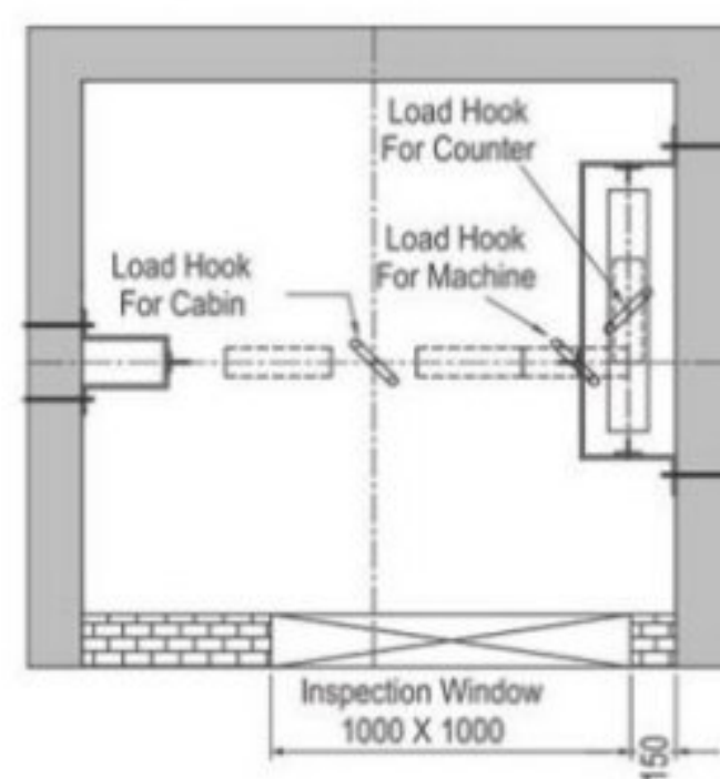
Lift Well Plan
