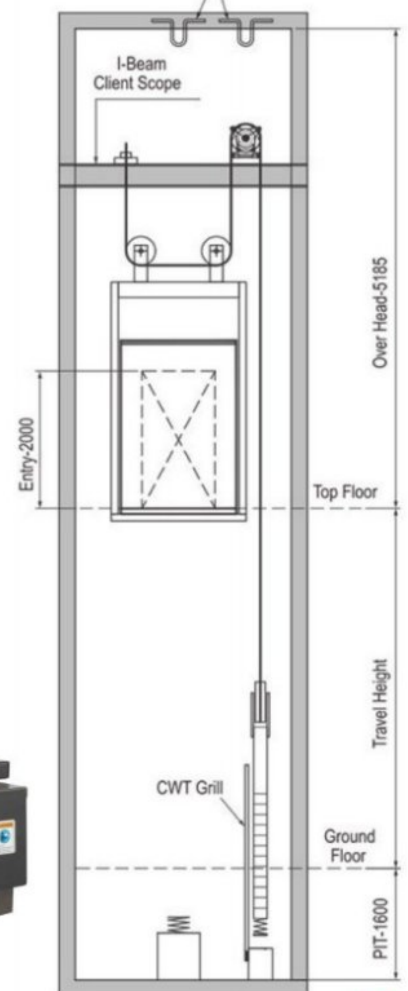
Lift Well Section View
