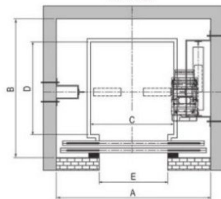
Lift Well Plan
